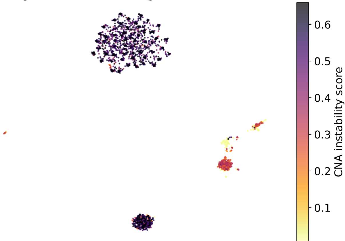
Fig 1E — CNA score (high = tumour cells)
